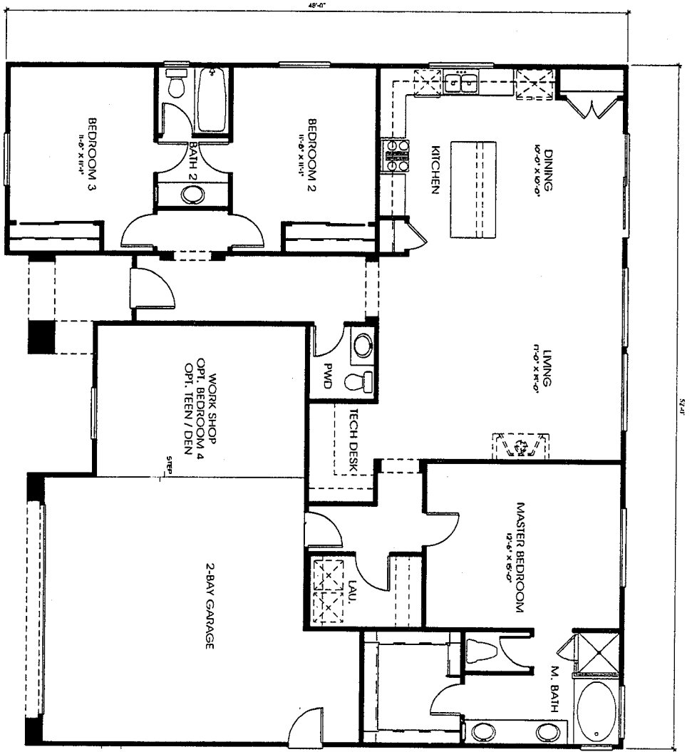
FLOOR PLAN 1,657 S.F.
